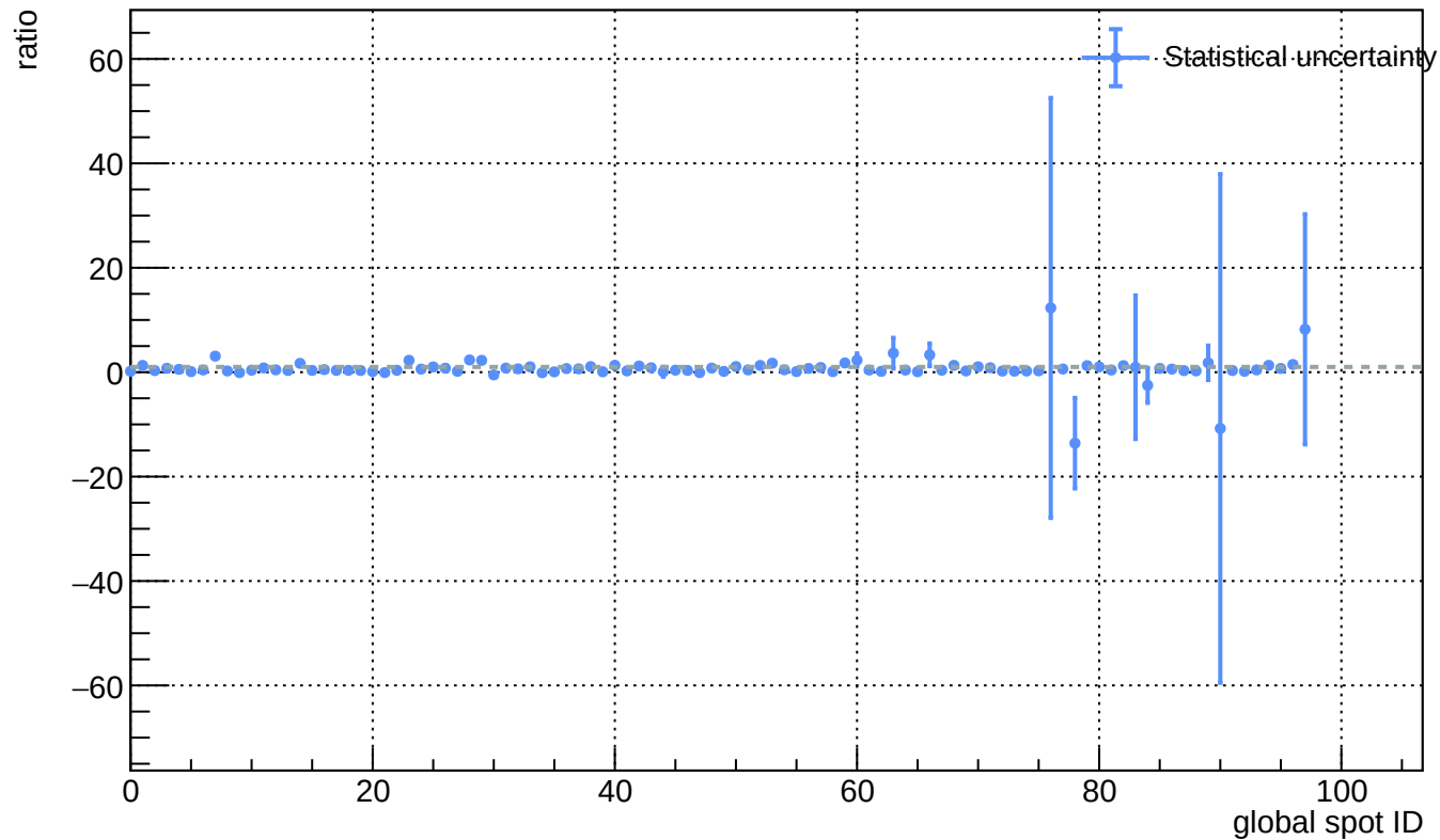
Sensor A1, v = 5\text{ V} - L(\text{ann\_100C\_25h}) / L(\text{before\_annealing})
