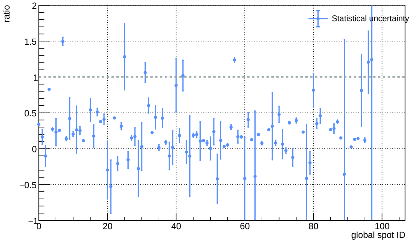
Sensor A1, v = 5\text{ V} - L(\text{ann\_125C\_25h}) / L(\text{before\_annealing})
