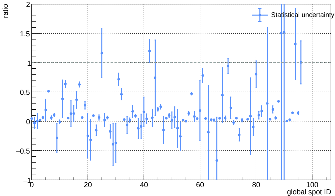
Sensor A1, v = 5 V - L(\text{ann\_150C\_25h}) / L(\text{before\_annealing})
