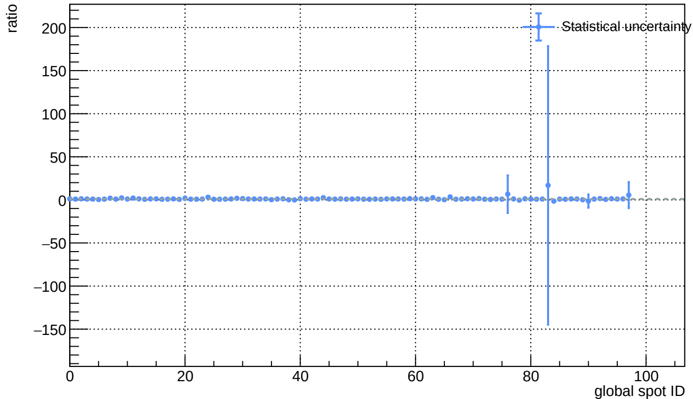
Sensor A1, v = 5 V - L(\text{ann\_75C\_5h}) / L(\text{before\_annealing})
