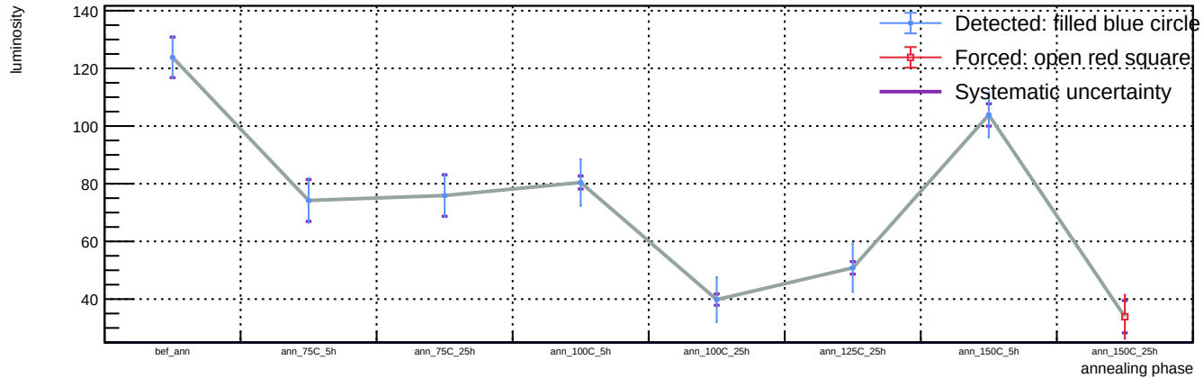
Sensor A1, v = 5 V, representative T = 23 C (max available) - Spot 19: luminosity vs phase
