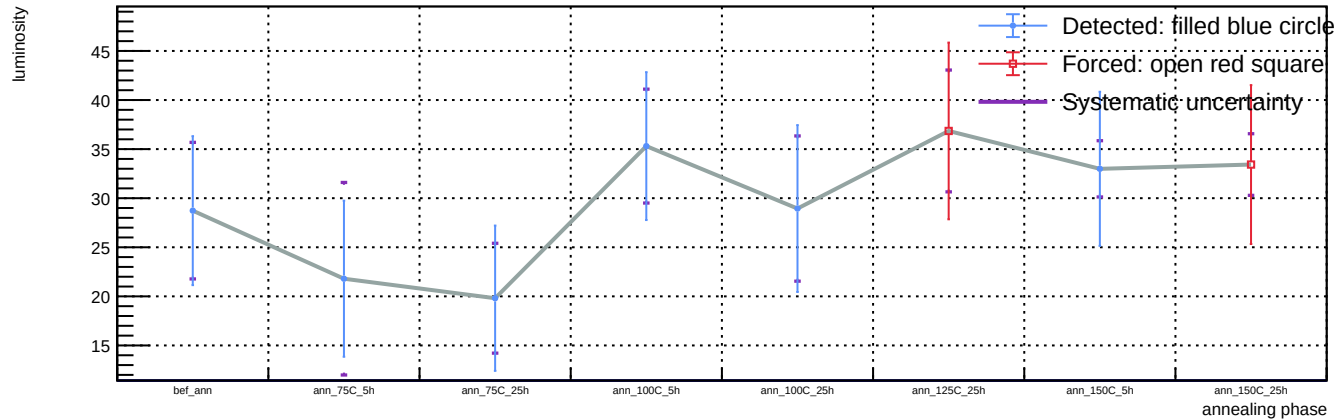
Sensor A1, v = 5 V, representative T = 23 C (max available) - Spot 25: luminosity vs phase
