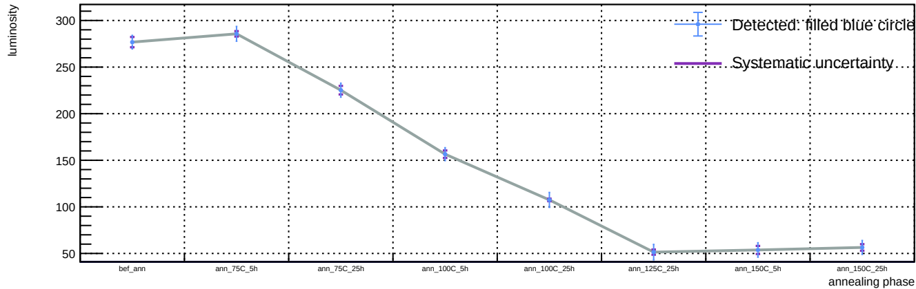
Sensor A1, v = 5 V, representative T = 23 C (max available) - Spot 45: luminosity vs phase
