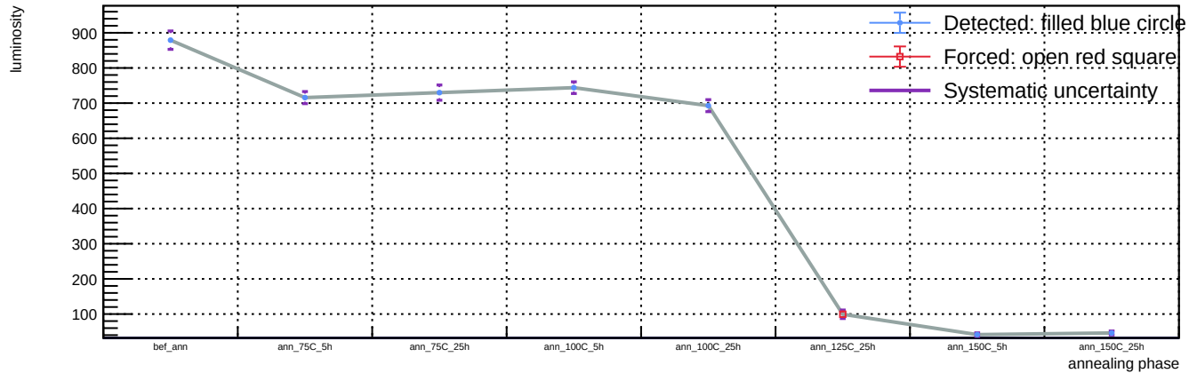
Sensor A1, v = 5 V, representative T = 23 C (max available) - Spot 48: luminosity vs phase
