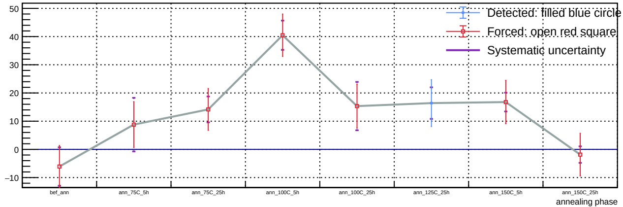
Sensor A1, v = 5 V, representative T = 23 C (max available) - Spot 84: luminosity vs phase
