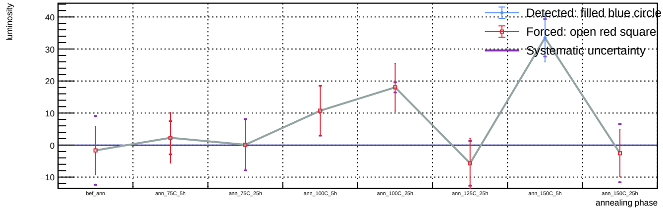
Sensor A1, v = 5 V, representative T = 23 C (max available) - Spot 90: luminosity vs phase
