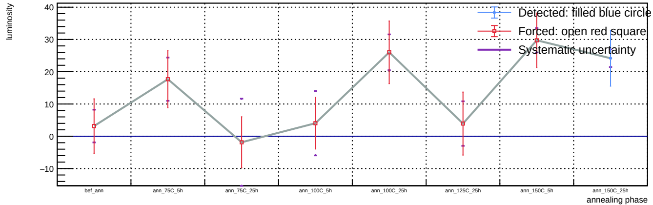
Sensor A1, v = 5 V, representative T = 23 C (max available) - Spot 97: luminosity vs phase
