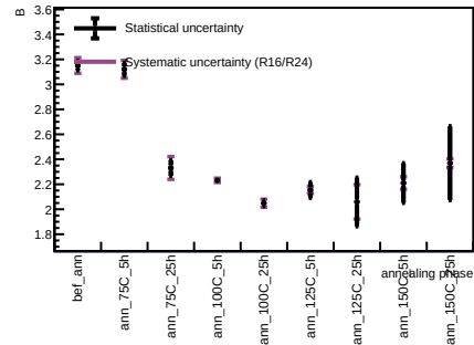
Sensor B1, T = 20 C - Spot 53
