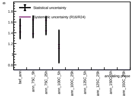
Sensor B1, T = 20 C - Spot 49
