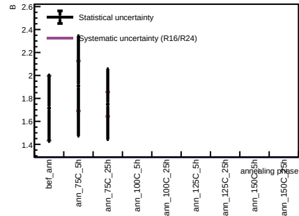
Sensor B1, T = 20 C - Spot 50
