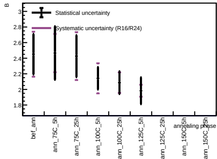
Sensor B1, T = 20 C - Spot 48
