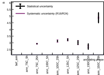
Sensor B1, T = 20 C - Spot 78
