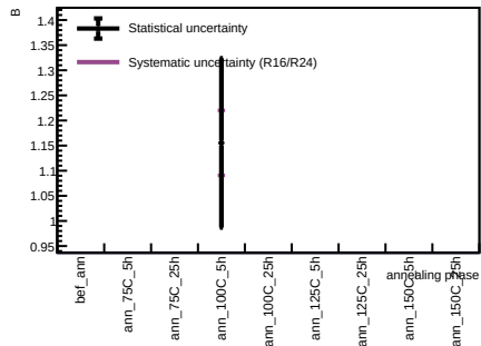
Sensor B1, T = 20 C - Spot 81
