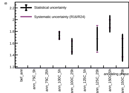
Sensor B1, T = 20 C - Spot 83
