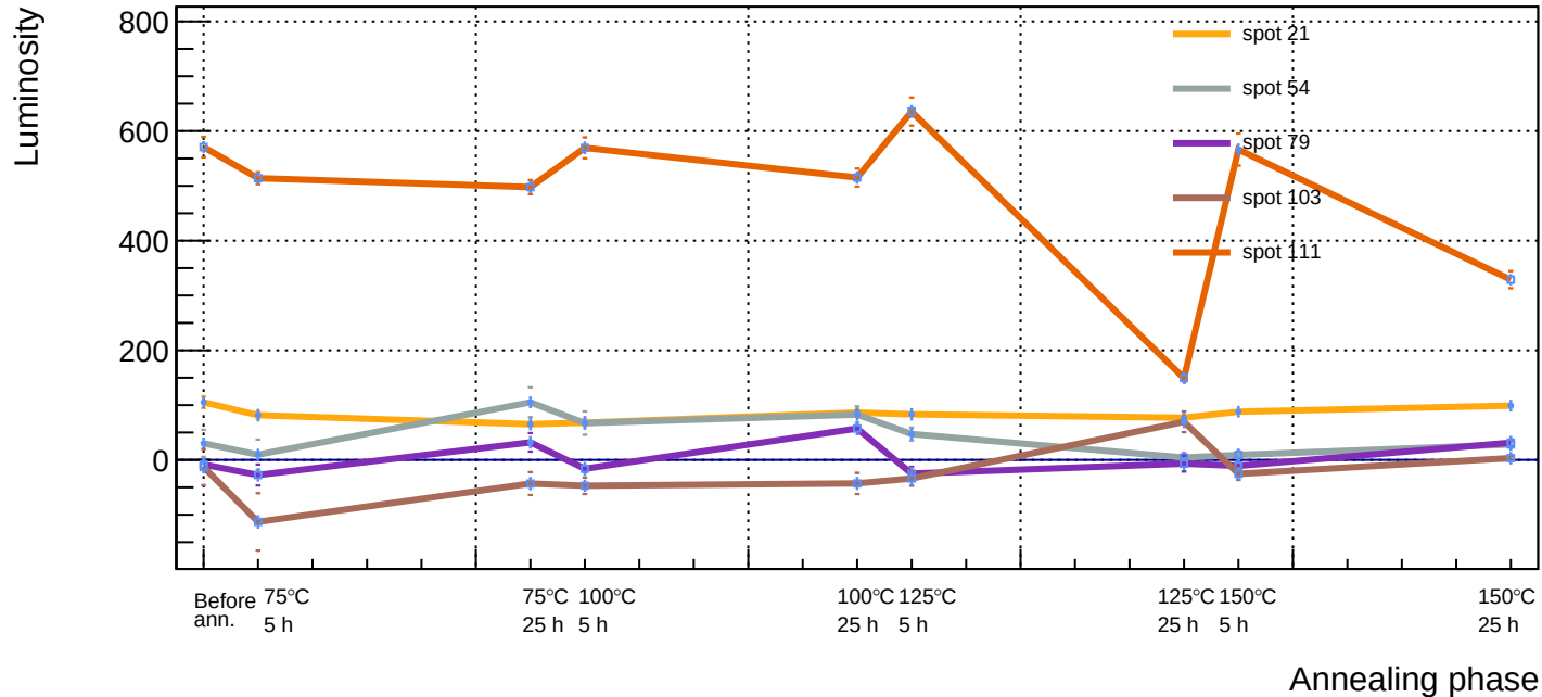
Sensor B1, T = 20\text{ C} , v_{\text{over}} = 5\text{ V} - Approximately constant hotspots
