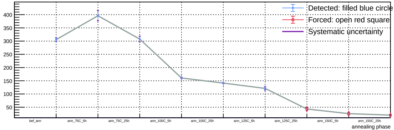
Sensor B1, T = 20\text{ C} , v_{\text{over}} = 5\text{ V} - Spot 1: luminosity vs phase
