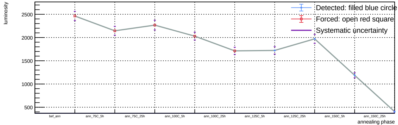
Sensor B1, T = 20\text{ C} , v_{\text{over}} = 5\text{ V} - Spot 101: luminosity vs phase
