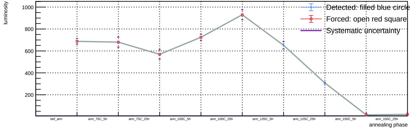
Sensor B1, T = 20\text{ C} , v_{\text{over}} = 5\text{ V} - Spot 102: luminosity vs phase
