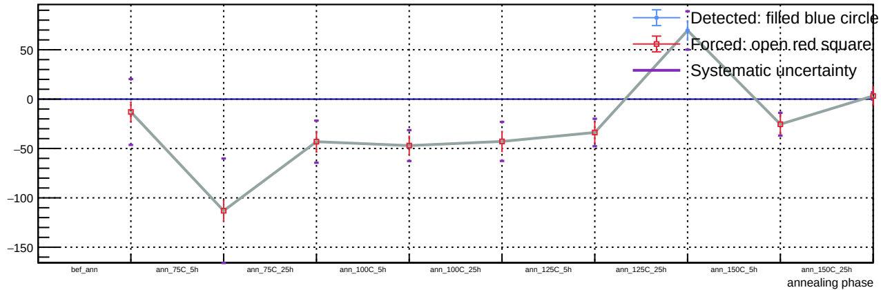
Sensor B1, T = 20\text{ C} , v_{\text{over}} = 5\text{ V} - Spot 103: luminosity vs phase
