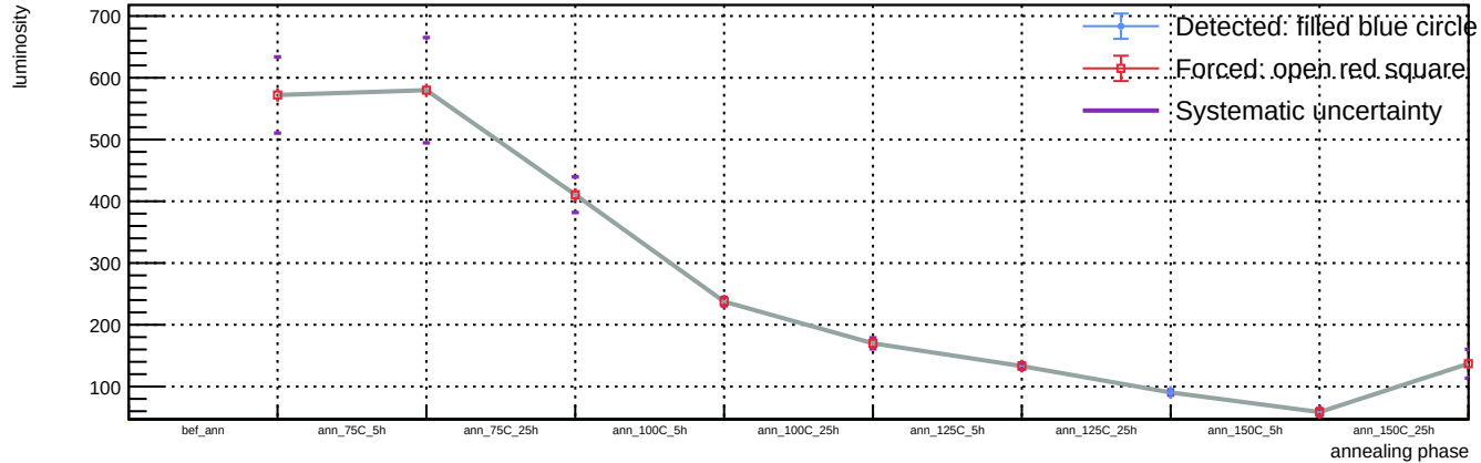
Sensor B1, T = 20\text{ C} , v_{\text{over}} = 5\text{ V} - Spot 104: luminosity vs phase
