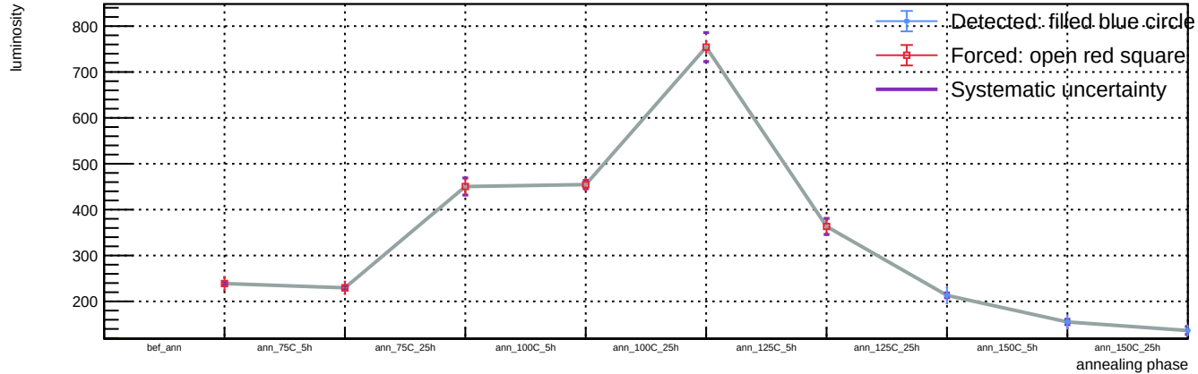
Sensor B1, T = 20\text{ C} , v_{\text{over}} = 5\text{ V} - Spot 106: luminosity vs phase
