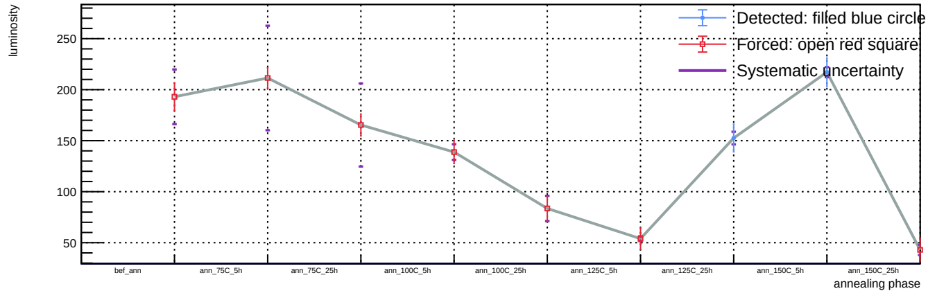
Sensor B1, T = 20\text{ C} , v_{\text{over}} = 5\text{ V} - Spot 108: luminosity vs phase
