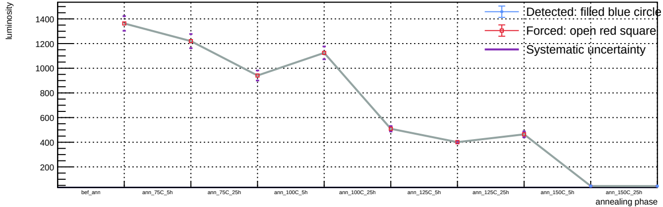
Sensor B1, T = 20\text{ C} , v_{\text{over}} = 5\text{ V} - Spot 112: luminosity vs phase
