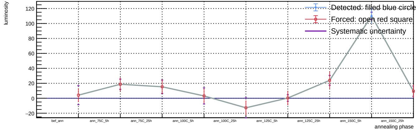
Sensor B1, T = 20\text{ C} , v_{\text{over}} = 5\text{ V} - Spot 113: luminosity vs phase
