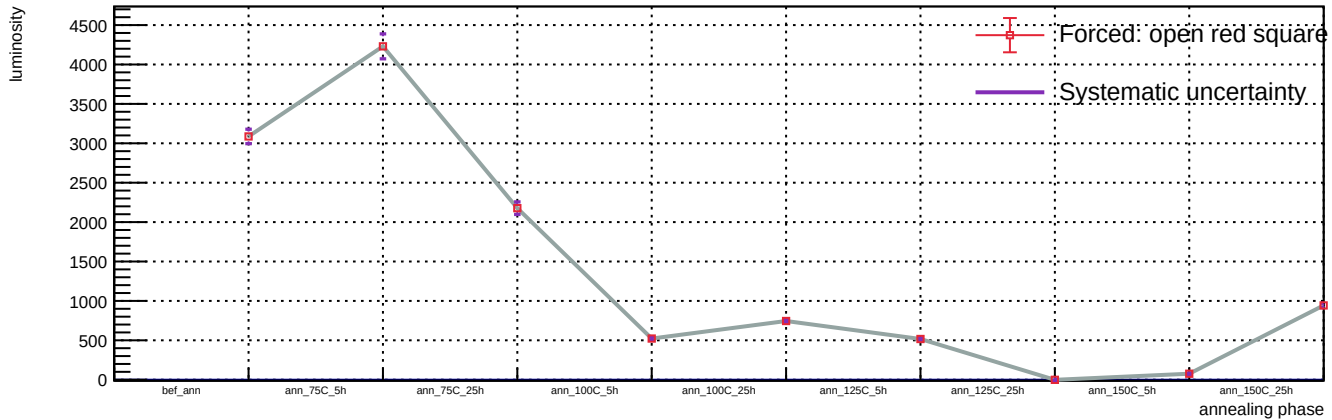
Sensor B1, T = 20\text{ C} , v_{\text{over}} = 5\text{ V} - Spot 115: luminosity vs phase
