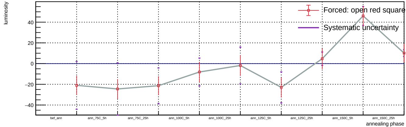
Sensor B1, T = 20\text{ C} , v_{\text{over}} = 5\text{ V} - Spot 116: luminosity vs phase
