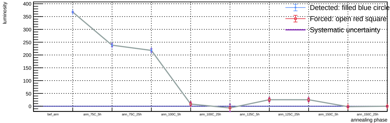
Sensor B1, T = 20\text{ C} , v_{\text{over}} = 5\text{ V} - Spot 13: luminosity vs phase
