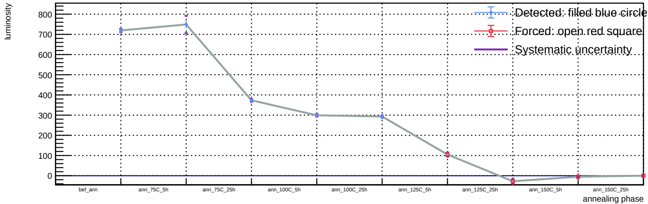
Sensor B1, T = 20\text{ C} , v_{\text{over}} = 5\text{ V} - Spot 17: luminosity vs phase
