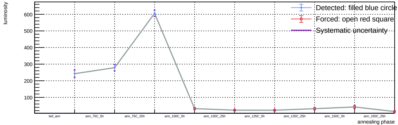
Sensor B1, T = 20\text{ C} , v_{\text{over}} = 5\text{ V} - Spot 2: luminosity vs phase
