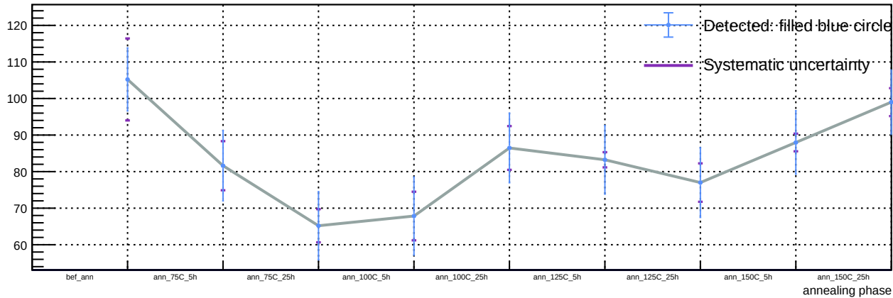
Sensor B1, T = 20\text{ C} , v_{\text{over}} = 5\text{ V} - Spot 21: luminosity vs phase
