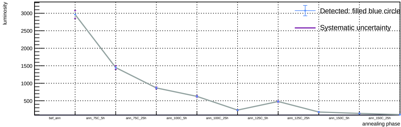
Sensor B1, T = 20\text{ C} , v_{\text{over}} = 5\text{ V} - Spot 23: luminosity vs phase
