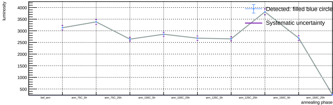
Sensor B1, T = 20\text{ C} , v_{\text{over}} = 5\text{ V} - Spot 26: luminosity vs phase
