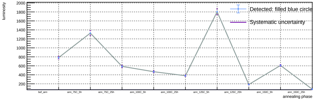
Sensor B1, T = 20\text{ C} , v_{\text{over}} = 5\text{ V} - Spot 29: luminosity vs phase
