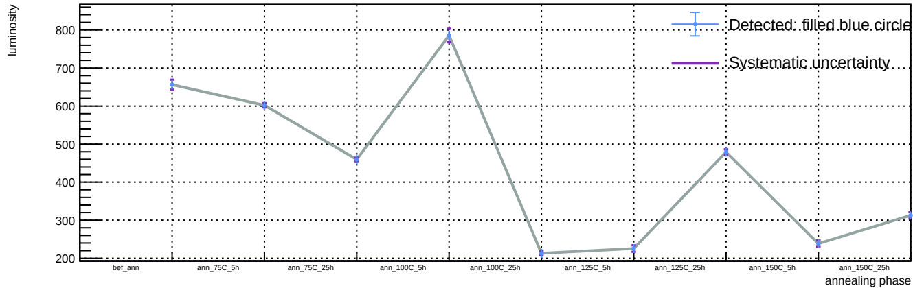
Sensor B1, T = 20\text{ C} , v_{\text{over}} = 5\text{ V} - Spot 31: luminosity vs phase
