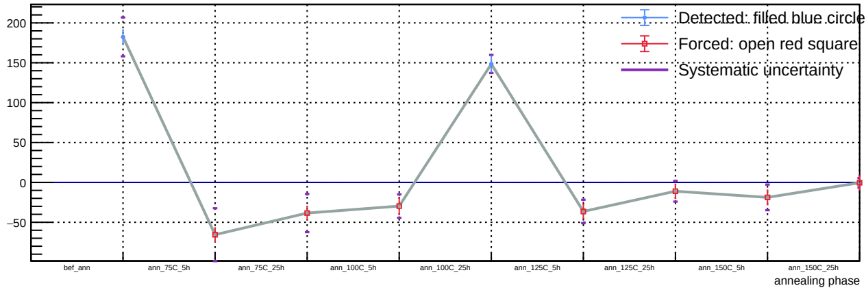
Sensor B1, T = 20\text{ C} , v_{\text{over}} = 5\text{ V} - Spot 35: luminosity vs phase
