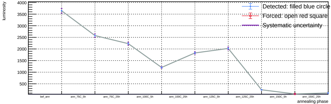
Sensor B1, T = 20\text{ C} , v_{\text{over}} = 5\text{ V} - Spot 36: luminosity vs phase
