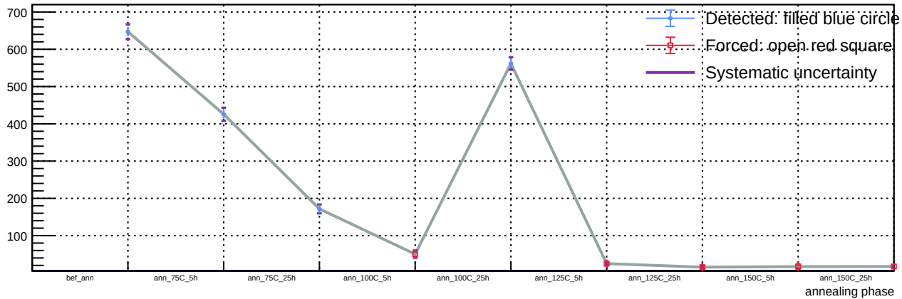
Sensor B1, T = 20\text{ C} , v_{\text{over}} = 5\text{ V} - Spot 37: luminosity vs phase
