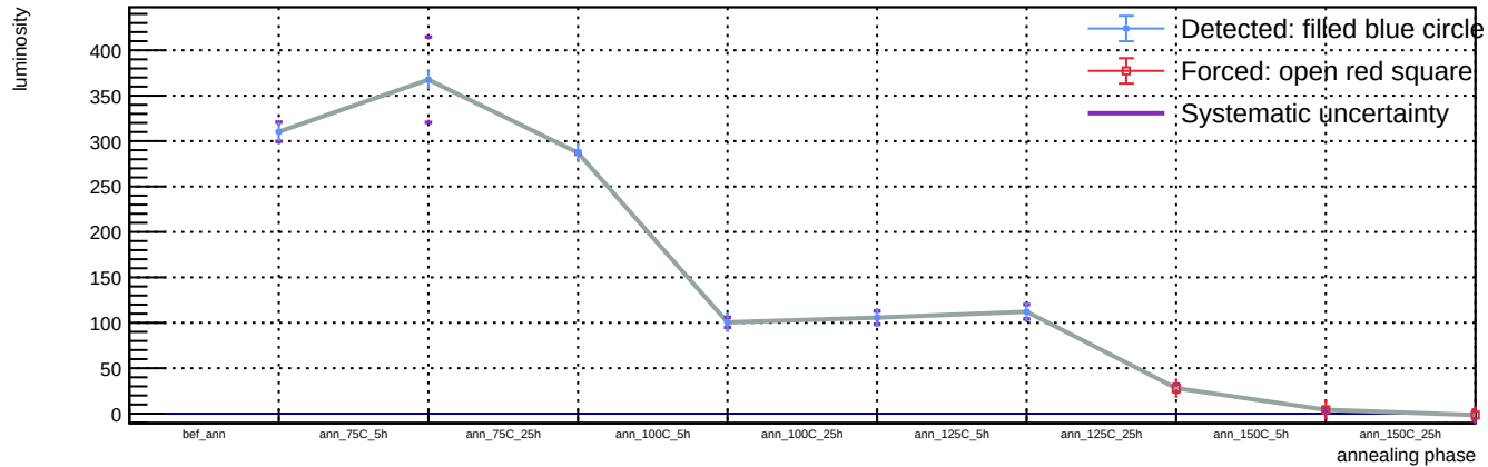
Sensor B1, T = 20\text{ C} , v_{\text{over}} = 5\text{ V} - Spot 4: luminosity vs phase
