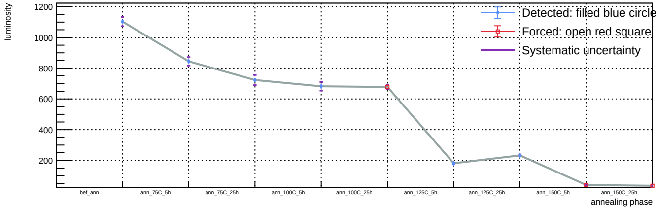
Sensor B1, T = 20\text{ C} , v_{\text{over}} = 5\text{ V} - Spot 42: luminosity vs phase
