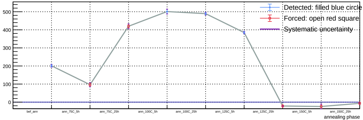
Sensor B1, T = 20\text{ C} , v_{\text{over}} = 5\text{ V} - Spot 43: luminosity vs phase
