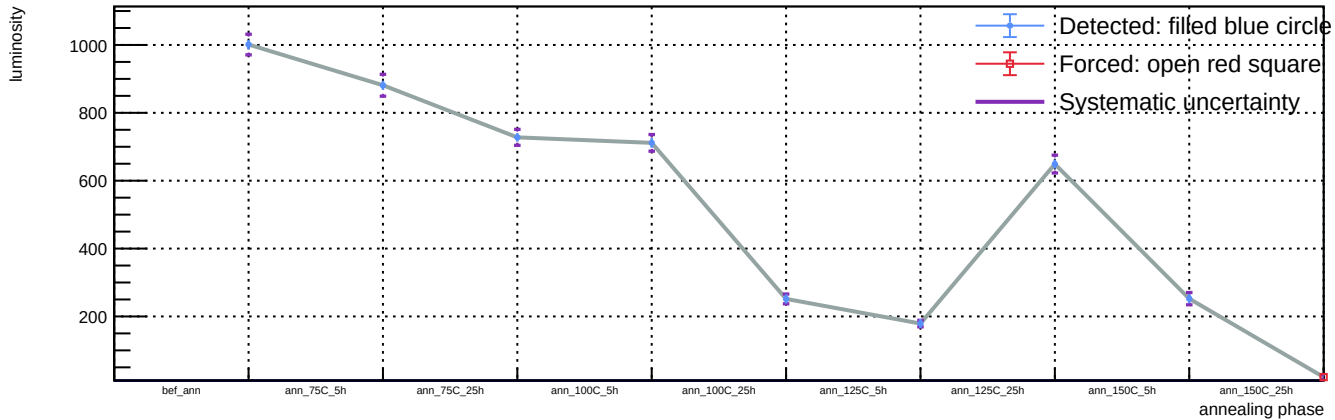
Sensor B1, T = 20\text{ C} , v_{\text{over}} = 5\text{ V} - Spot 45: luminosity vs phase
