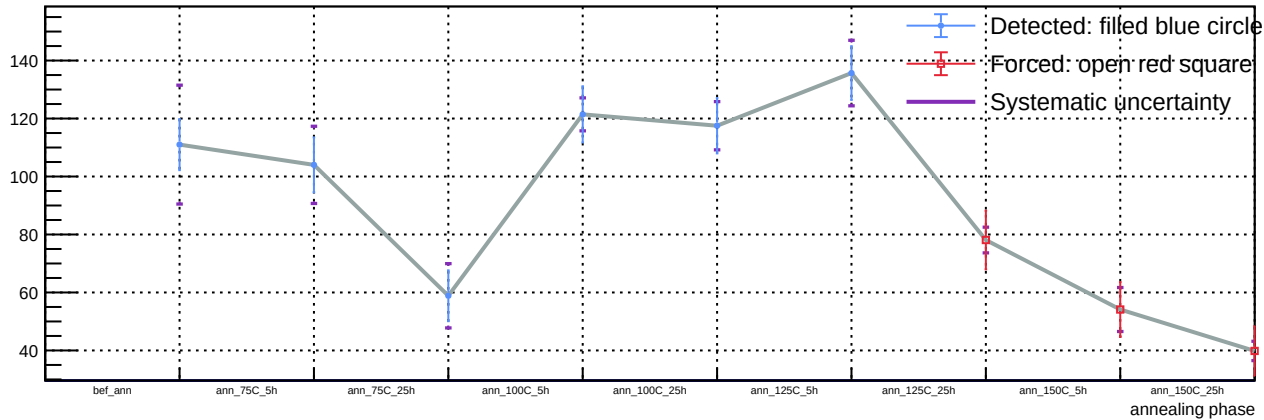
Sensor B1, T = 20\text{ C} , v_{\text{over}} = 5\text{ V} - Spot 46: luminosity vs phase
