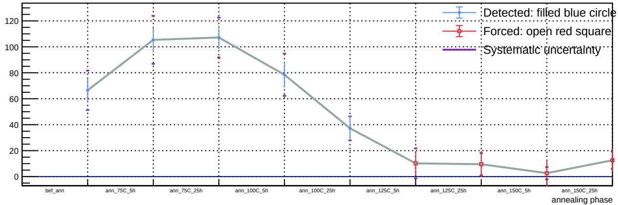
Sensor B1, T = 20\text{ C} , v_{\text{over}} = 5\text{ V} - Spot 47: luminosity vs phase
