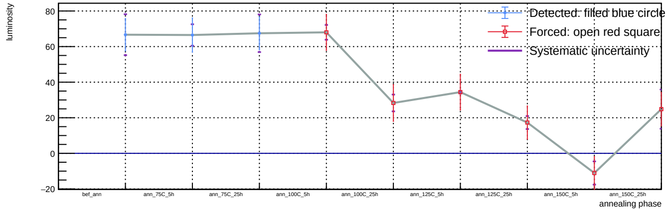
Sensor B1, T = 20\text{ C} , v_{\text{over}} = 5\text{ V} - Spot 50: luminosity vs phase
