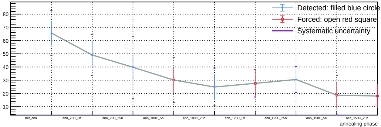
Sensor B1, T = 20\text{ C} , v_{\text{over}} = 5\text{ V} - Spot 51: luminosity vs phase
