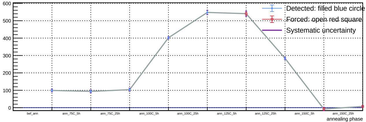
Sensor B1, T = 20\text{ C} , v_{\text{over}} = 5\text{ V} - Spot 52: luminosity vs phase
