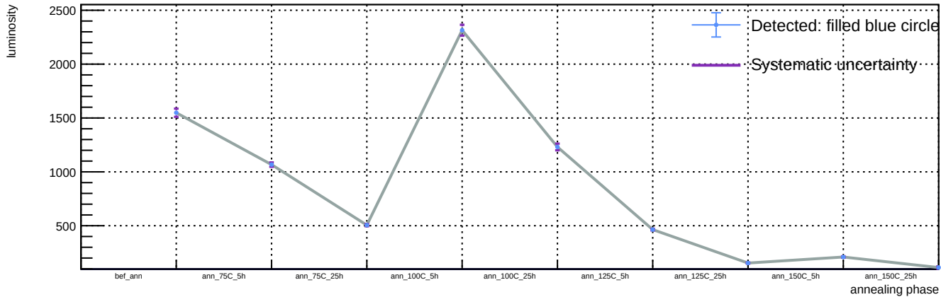
Sensor B1, T = 20\text{ C} , v_{\text{over}} = 5\text{ V} - Spot 53: luminosity vs phase
