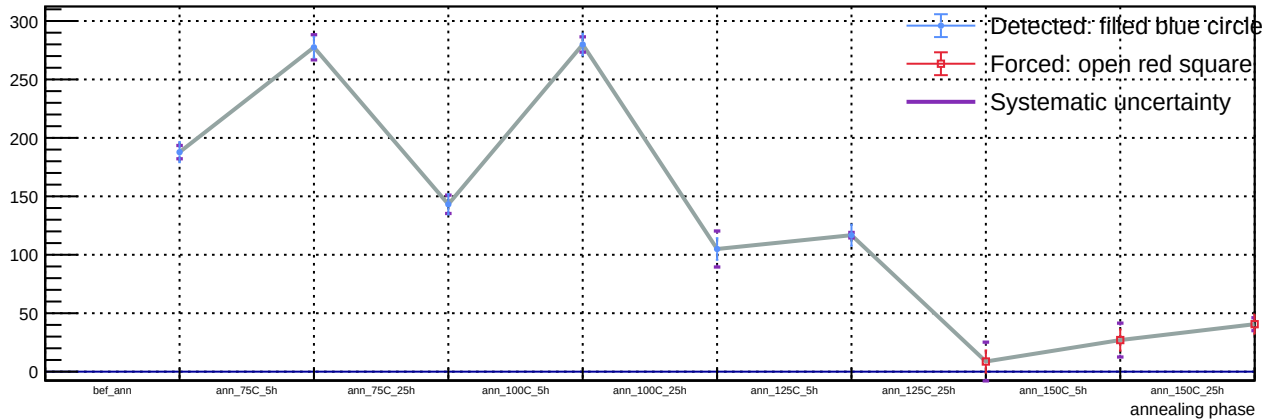
Sensor B1, T = 20\text{ C} , v_{\text{over}} = 5\text{ V} - Spot 58: luminosity vs phase
