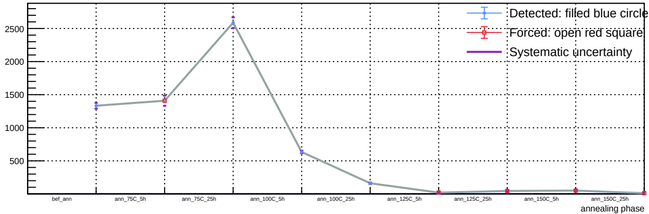
Sensor B1, T = 20\text{ C} , v_{\text{over}} = 5\text{ V} - Spot 59: luminosity vs phase
