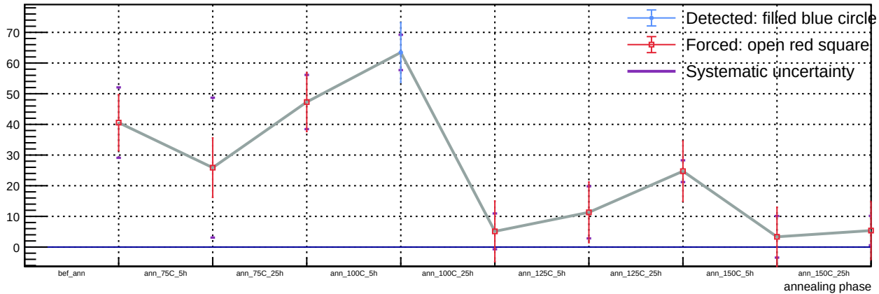
Sensor B1, T = 20\text{ C} , v_{\text{over}} = 5\text{ V} - Spot 62: luminosity vs phase
