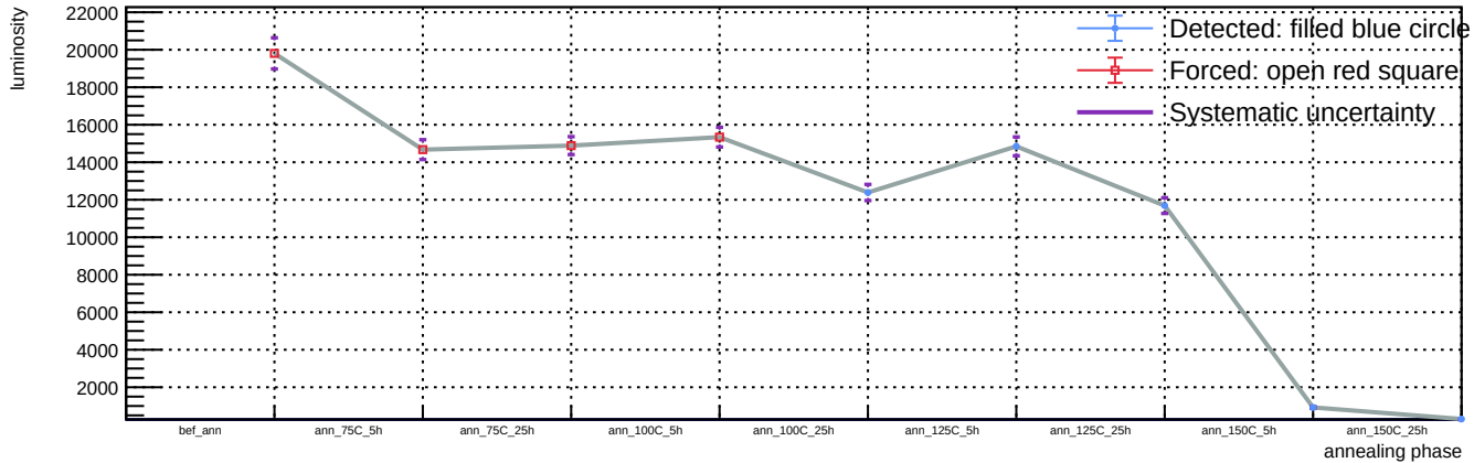
Sensor B1, T = 20\text{ C} , v_{\text{over}} = 5\text{ V} - Spot 63: luminosity vs phase
